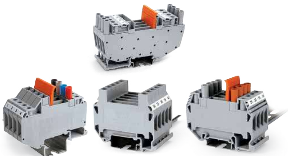
Circuit examples with RST6
