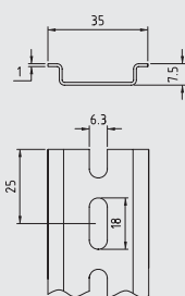
TH35-7.5
