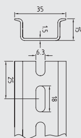
TH35-15
