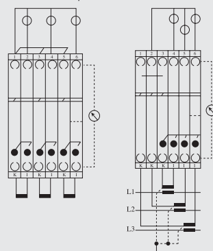
Circuit examples with RST6,RTT6
