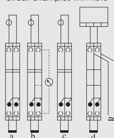
Circuit examples with RST6
