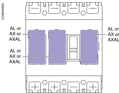
AXAL electrical auxiliaries on Ezc250.
