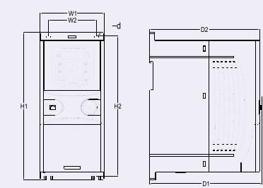
Wall mounting of 0.75~2.2kW VFDs
