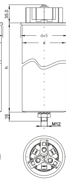
Three-phase capacitor with d = 85 mm
