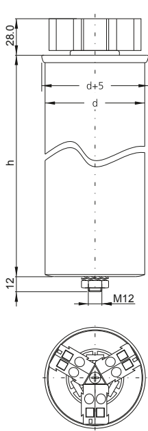
Three-phase capacitor with d = 60/70 mm
