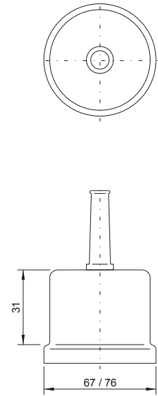
Plastic cap and rubber sleeve LKK 60/70 for capacitors with:
