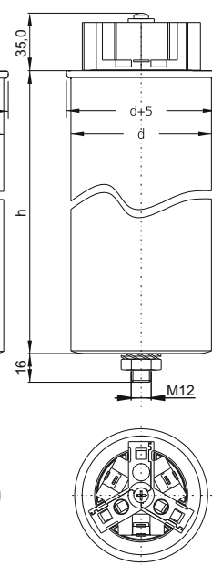
Single-phase capacitor with d = 85 mm
